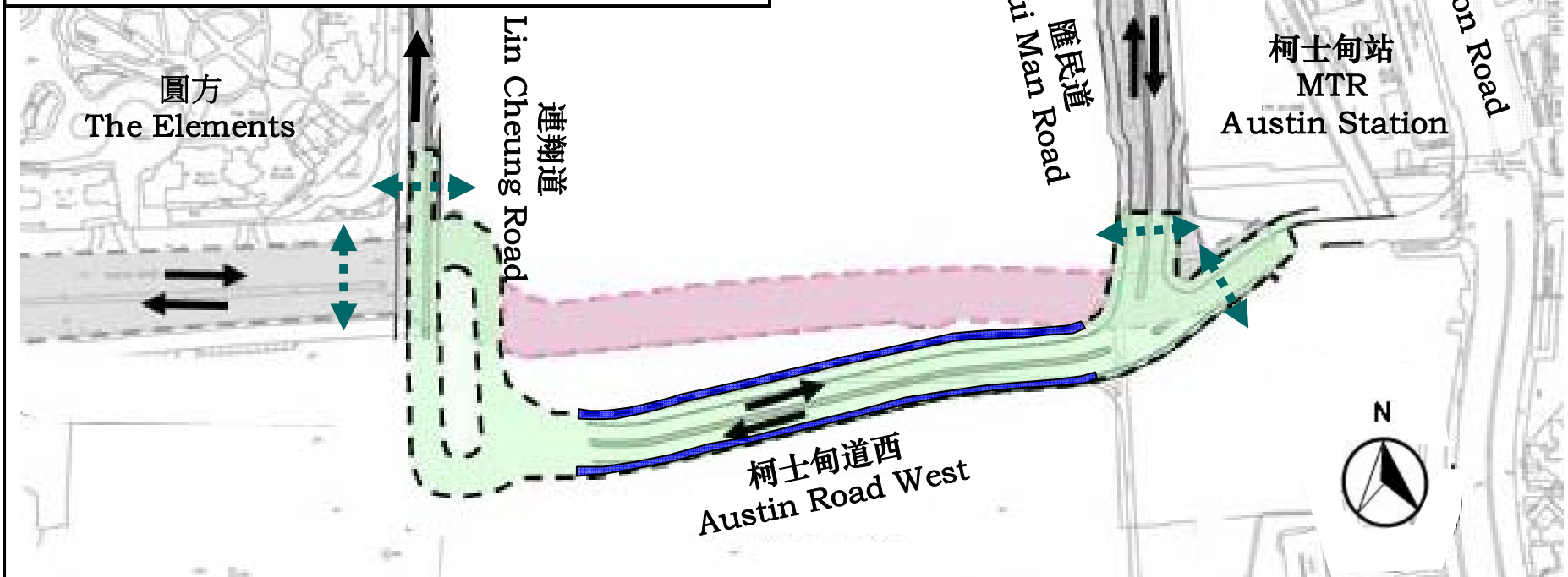
2011年10月20日柯士甸道西改行臨時行車橋及有蓋行人通道 Realignment of Austin Road West to temporary steel bridge and covered walkway on 20 October 2011
